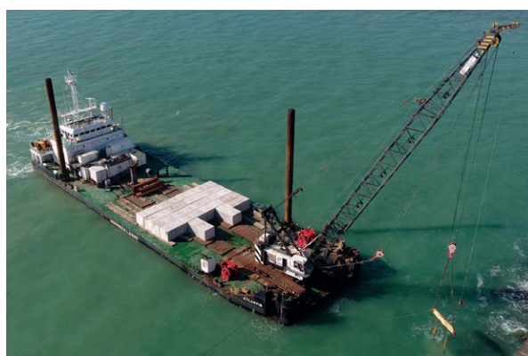
Multipurpose vessel
